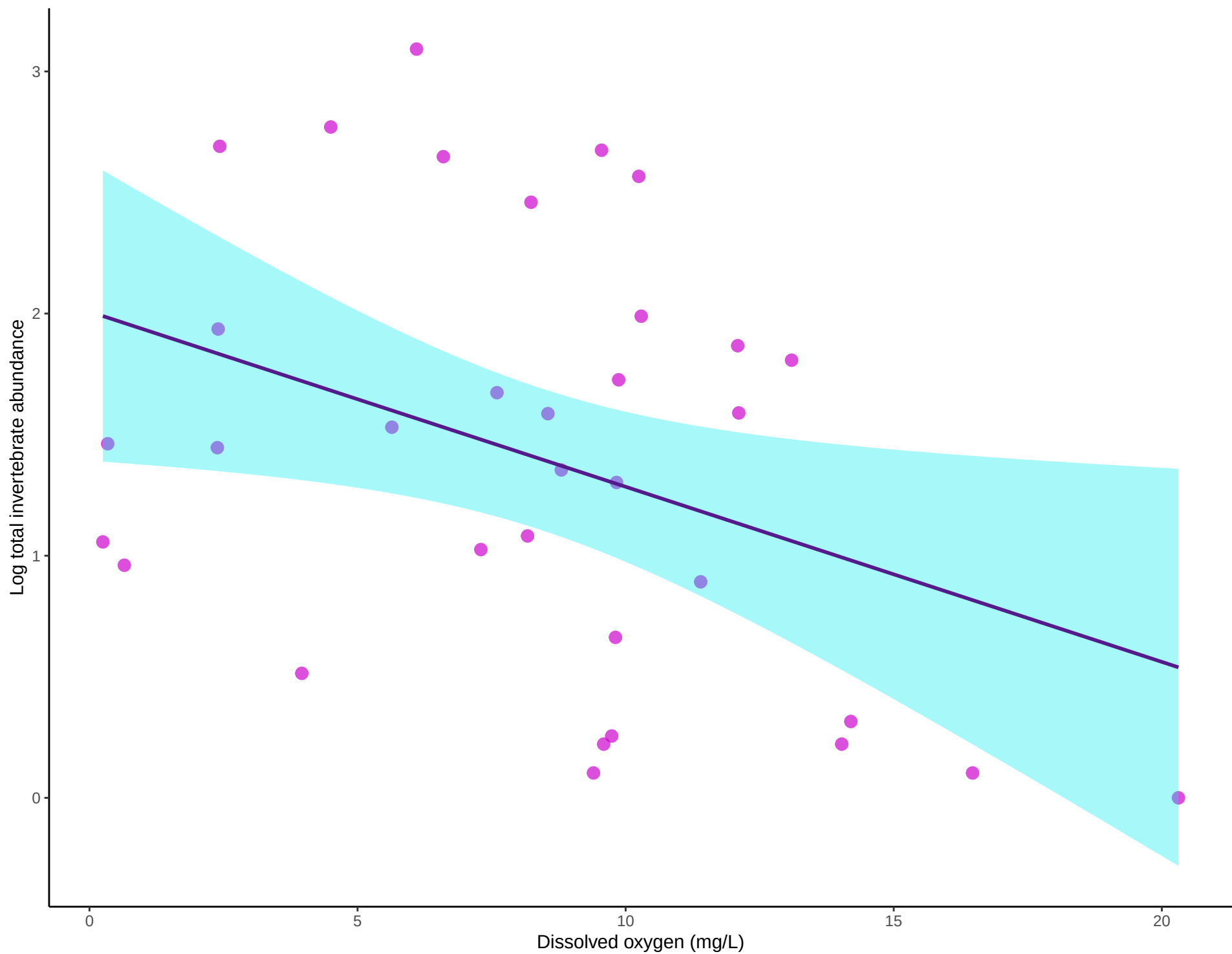
Relationship between DO + total invertebrate abundance
